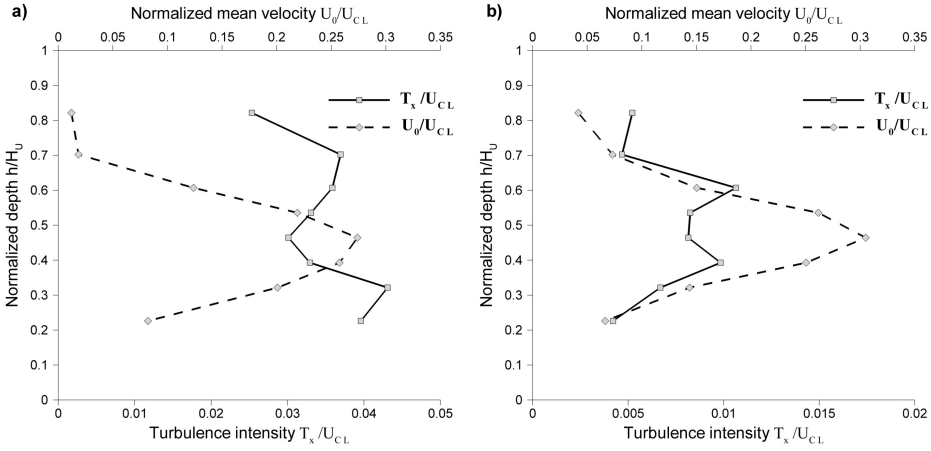
Fig. 11. Normalized turbulence and mean velocity at the 0.5 pipe diameter distance from the culvert entrance for (a) the vertical headwall case and (b) the projecting barrel case
