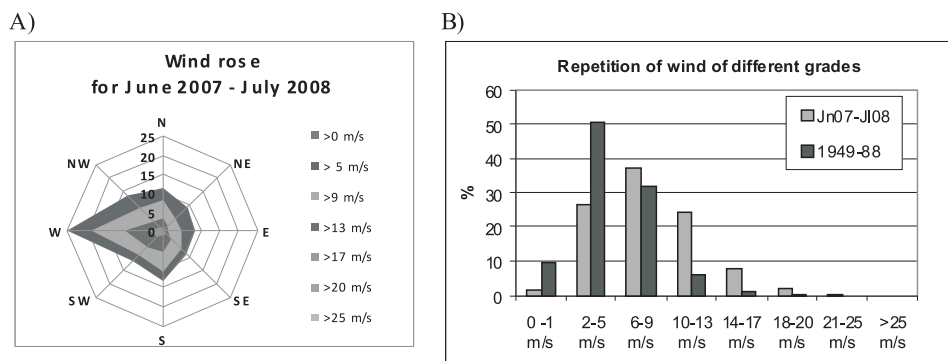
Fig. 9. Wind statistics for June 2007–July 2008 (A) for the off-shore station at the oil platform D6, in comparison with historical wind statistics for 1949–1988 (B)
