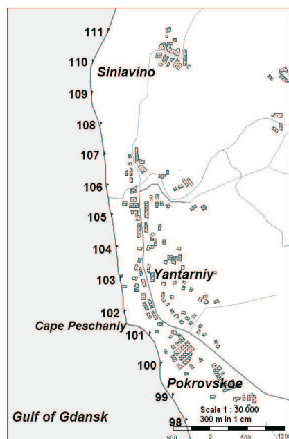
Fig. 6. Ground-based monitoring network of the study area, supported by State organization “Baltberegozastita”. Numbers indicate the location of monitoring profiles
