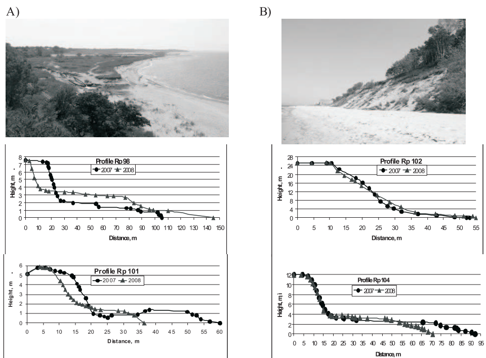
Fig. 7. Views and characteristic altitude profiles for 2007–2008 for the Bay of Pokrovskoe (A) and the cliff in Yantarniy (B)
