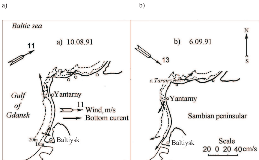
Fig. 8. Synchronous distribution of the near-bed currents during the acute-angle directional wind to the Sambian shore (Babakov 2003)
