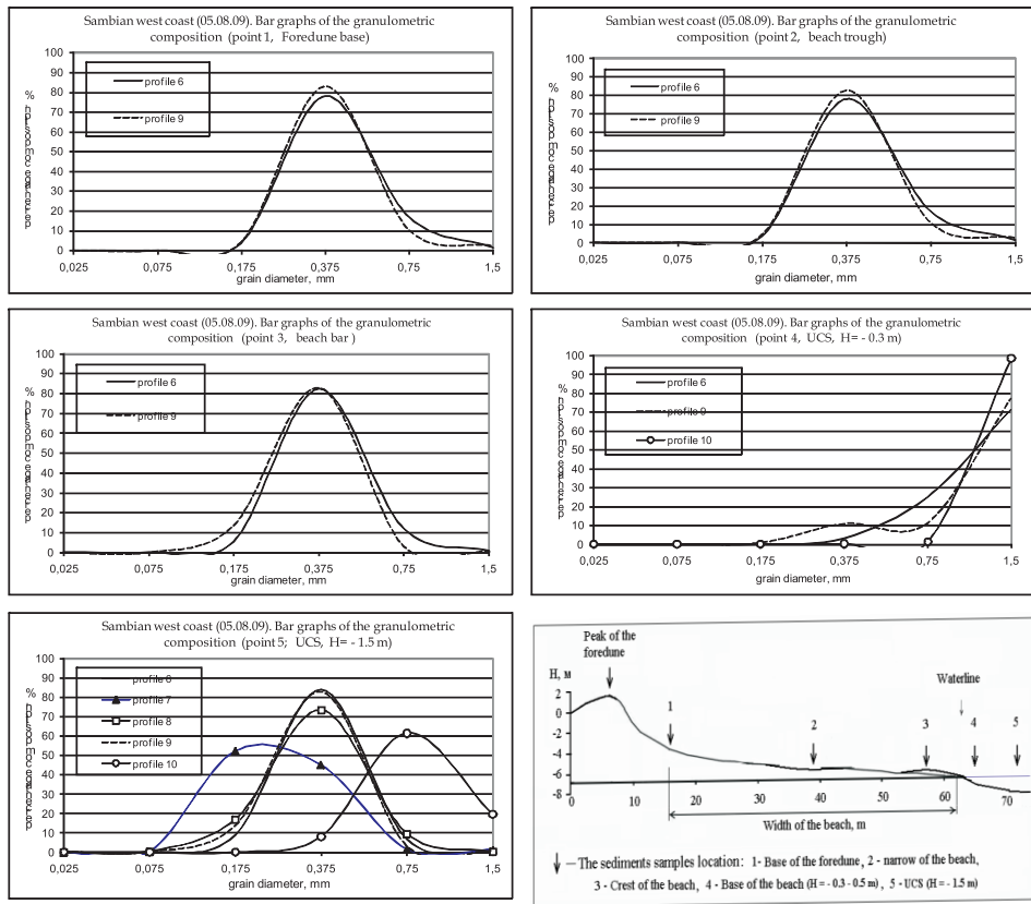
Fig. 11. Grain-size distributions for the deposits, detected along the Sambian coast (Yantarny – Baltiysk, profiles 6–10) for each point (1–5) of the profile
