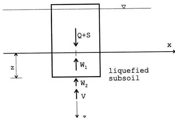
Fig. 7. Sinking of breakwater in liquefied subsoil
