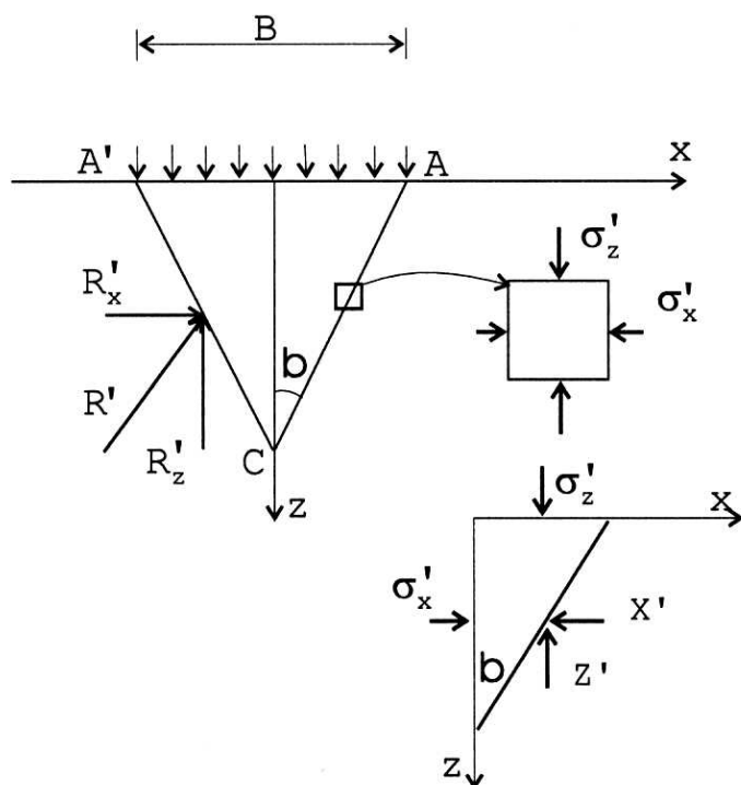
Fig. 5. Simplified stress state at surface AC
