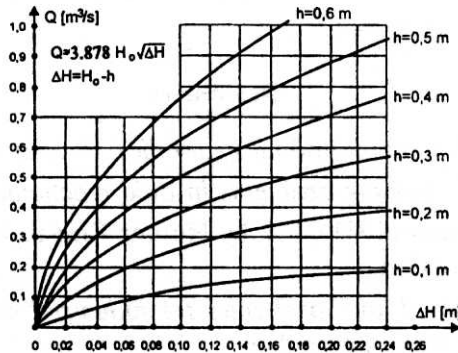
Fig. 15. Two-point characteristics for flume FG
