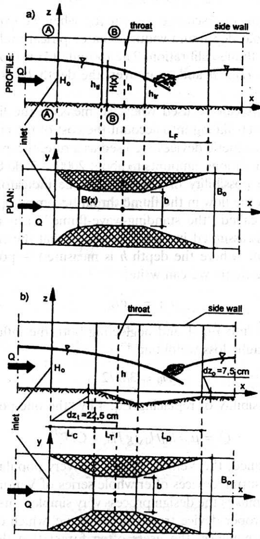
Fig. 1. General scheme of the Venturi (a) and Parshall (b) flume
