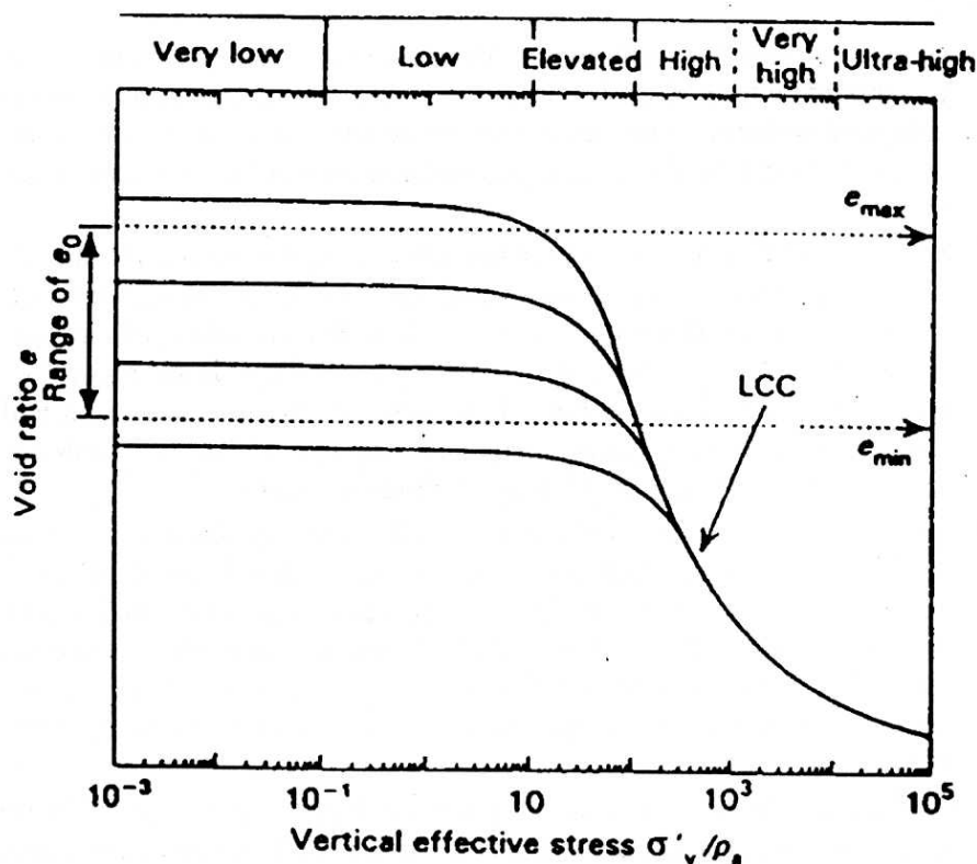
Fig. 6. Conceptual interpretation of hydrostatic and one-dimensional compression for freshly deposited cohesionless soils ( e_{\max} and e_{\min} are index properties defined by ASTM D4253-93 and D4254-91), (after Pestana and Whittle, 1995)
