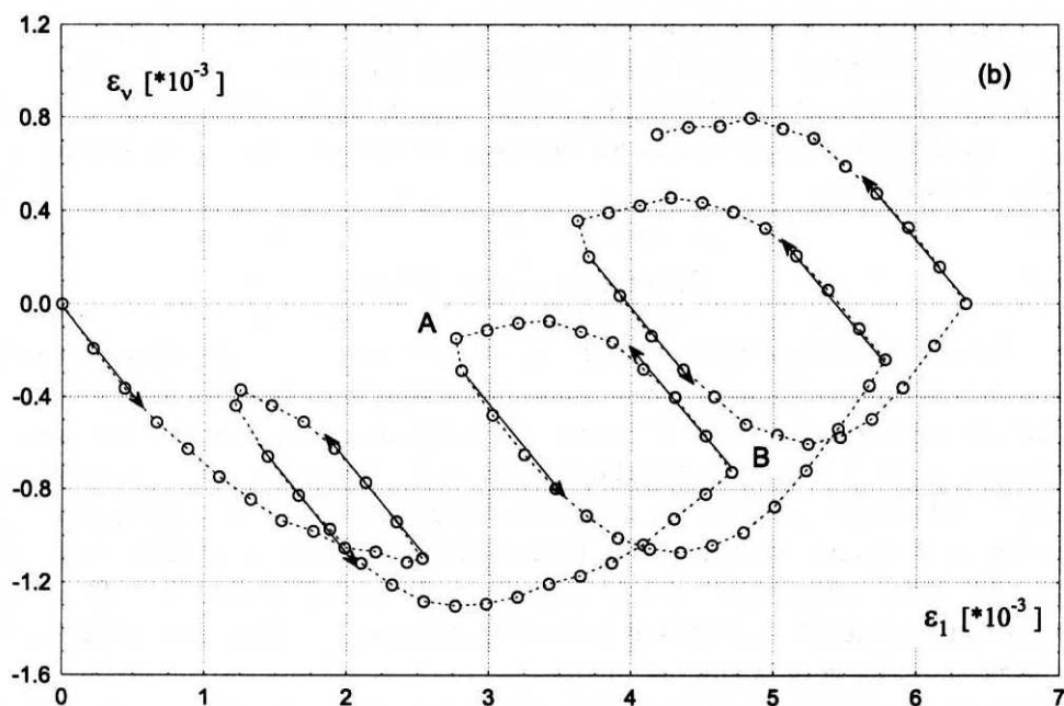
Fig. 1. Stress-strain and volume change behaviour of dense Lubiatowo sand in triaxial compression tests with several unloading-reloading cycles
